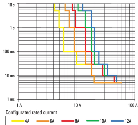
Tripping characteristic lag
